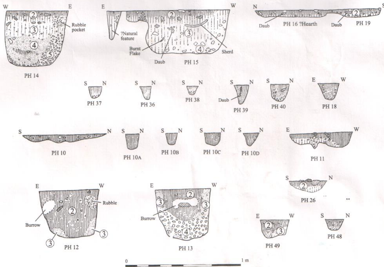
Figure 3.23. Wyke Down 2 (WD 2 1996): plan and sections of house 1 (M. Brudenell after M. Green).
