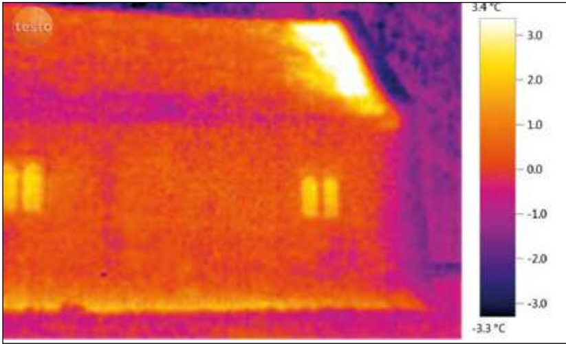
Thermal imaging showing the extent to which the underfloor heating lifts the temperature of floor level.
