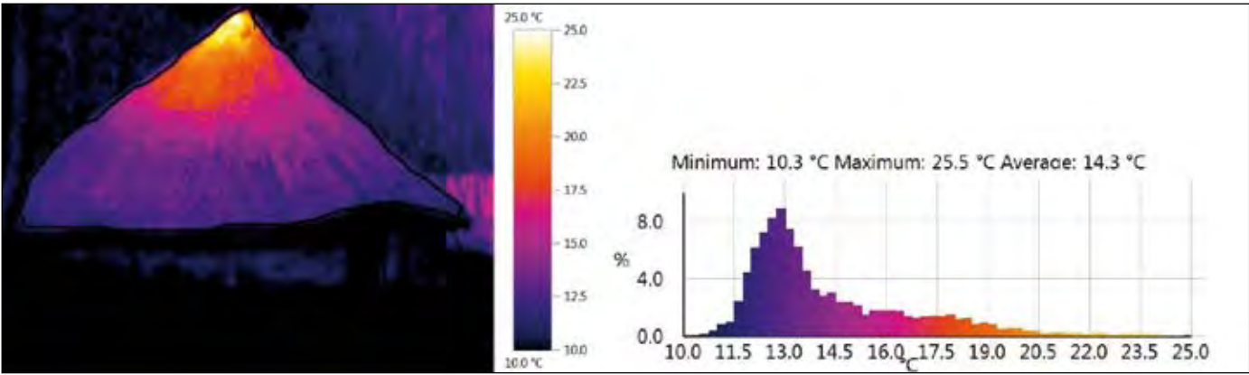
Fig 3. Thermal image taken 10:13AM.
