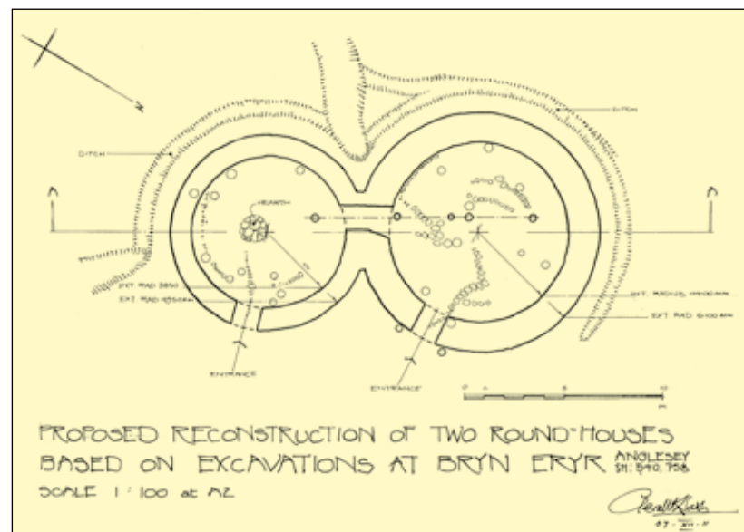
Ground plan of the Iron Age farmstead as used during the building work.
