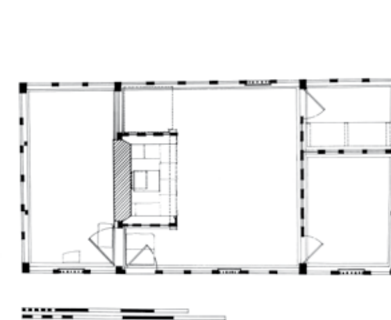
Abernodwydd farmhouse. Ground floor plan showing position of central fireplace, windows and door.
