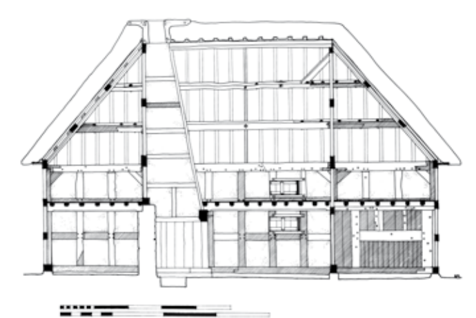
Section through Abernodwydd showing the location of the central fireplace and chimney.
