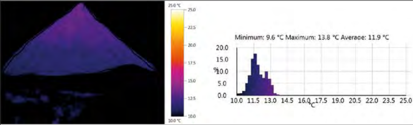
Fig 1. Thermal image taken 9:11AM.
