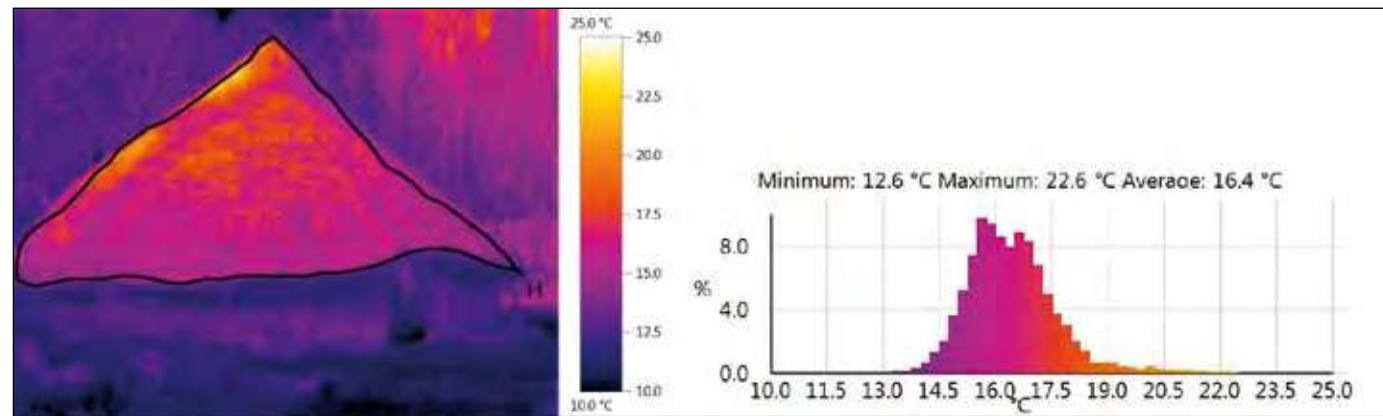
Fig 7. Thermal image taken 10:59AM.
