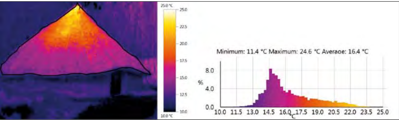
Fig 4. Thermal image taken 10:21AM.
